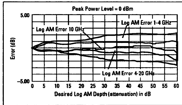
Figure 1-29. Typical Log AM Error (deviation from desired depth) at 25 °C for Carrier Frequencies between 1.0 and 20 GHz
