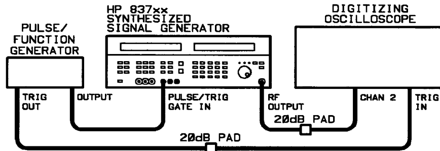
Figure 3-17. Pulse Width Test Setup
